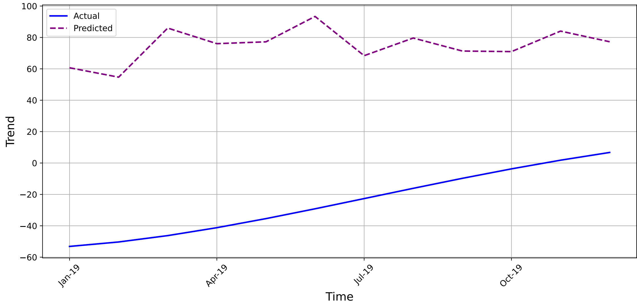
Botnet-ALL - Testing
